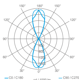
Optic 2x43°
