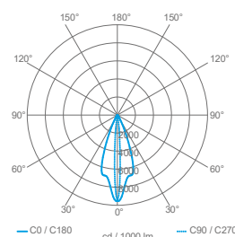
Optic 11°x39°
