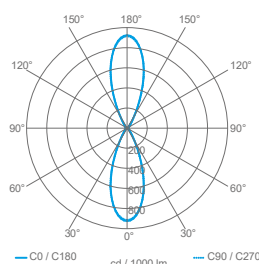
Optic 2x40°
