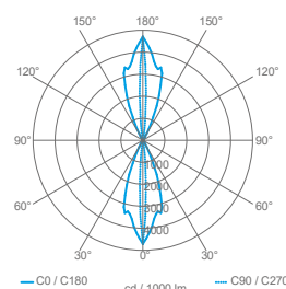
Optic 2x11°x39°
