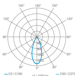
Optic 40°
